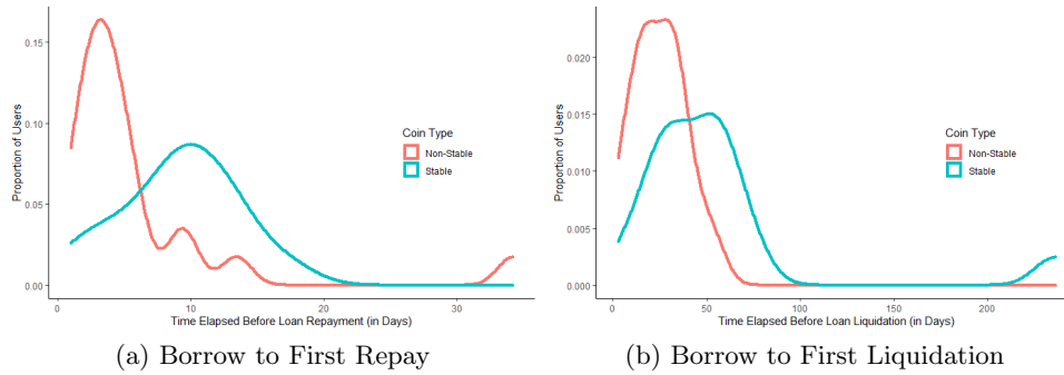
Fig. 3: Borrow to first repay and first liquidation analysis both show differences between stable and non-stablecoins.
