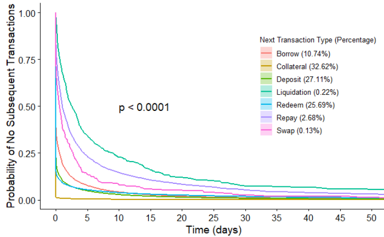
Fig. 1: Kaplan-Meier survival curves from a user’s deposits to their next transaction shows noticeable differences between which transactions users tend to make after a deposit.
